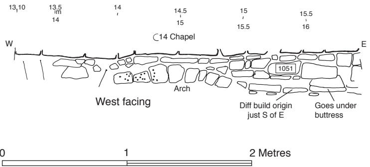
Section 108
