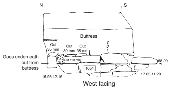
Section 110
